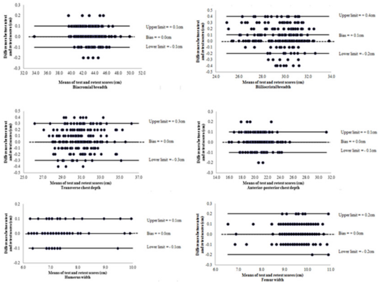
Figure 3: Bland and Altman plots summarising the 95% limits of agreement for the reliability of Biacromial and Biliochrystal Breadth, Transverse Chest and Anterior-Posterior Chest depth, Humerus and Femur width (cm).
