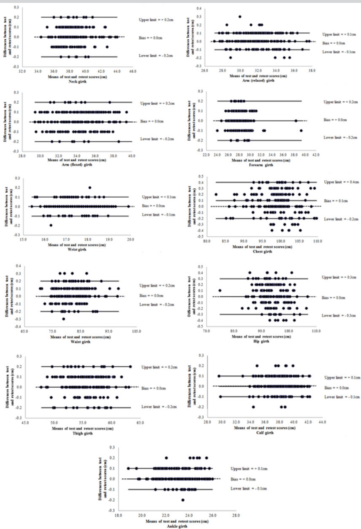
Figure 2: Bland and Altman plots summarising the 95% limits of agreement for the reliability of Neck, Arm (relaxed), Arm (flexed), Forearm, Thigh, Calf and Ankle girths (cm).
